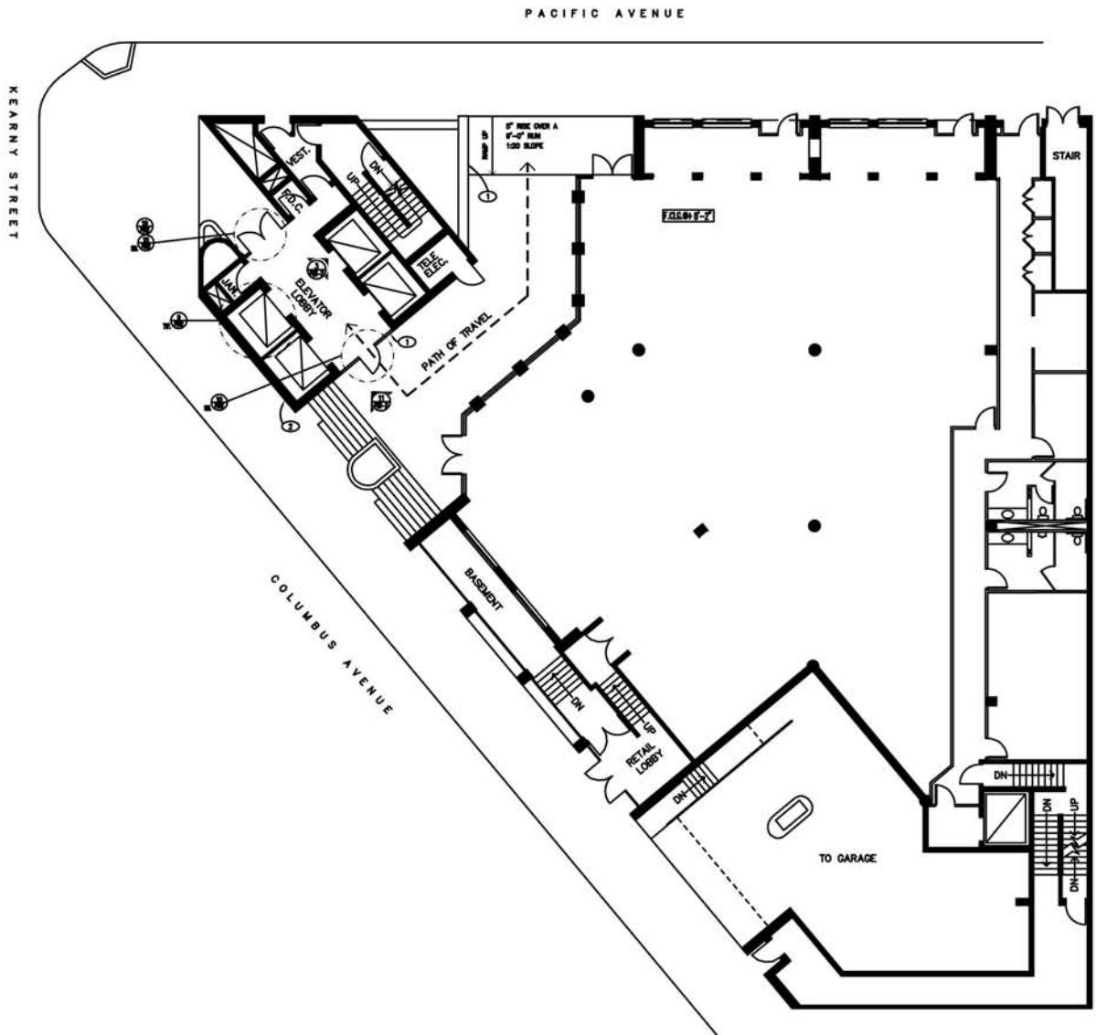
2 PATH OF TRAVEL, STREET LEVEL SCALE: 1/8" = 1'-0"
